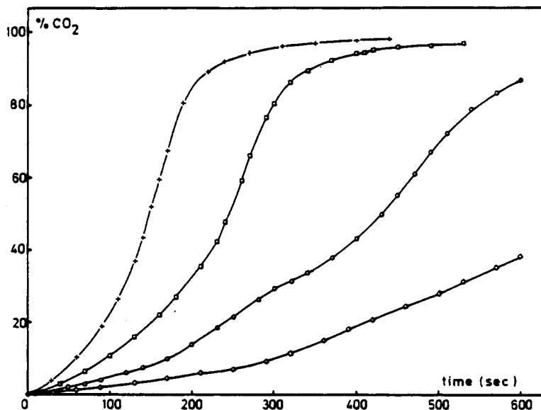
Fig. 5. \text{CO}_2 evolution curves; intrinsic catalytic effect of NMP and dioxane in formulations based on 100 parts MDI and 0.21 part 2MI: (+) 31 parts NMP; (□) 20 parts NMP and 15 parts dioxane; (○) 10 parts NMP and 30 parts dioxane; (◇) 48 parts dioxane.
