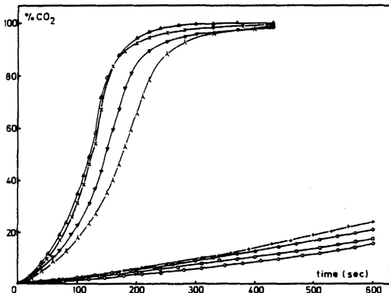
Fig. 4. CO 2 evolution curves; effect of NMP as cosolvent. No NMP added to 100 parts MDI, 46 parts H 2 O and 64 parts TCEP: (+) 2MI (0.21 part); (□) DABCO (0.29 part); (○) DMEA (0.42 part); (◇) no catalyst. 31 parts NMP added to 100 parts MDI, 31 parts H 2 O and 43 parts TCEP: (▽) 2MI (0.21 part); (△) DABCO (0.29 part); (X) DMEA (0.42 part); (▲) no catalyst.
