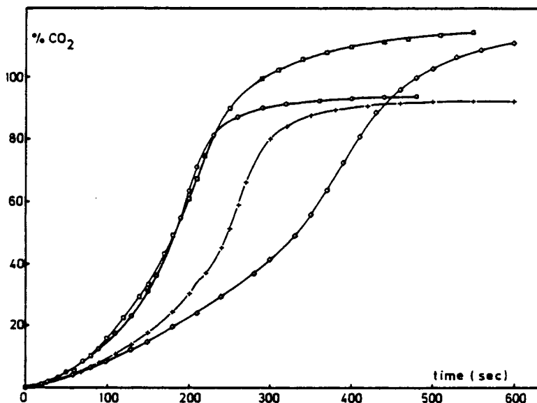
Fig. 6. \text{CO}_2 evolution curves; effect of the TCEP/NMP ratio in formulations containing 100 parts MDI and 31 parts water. TCEP/NMP: (+) 1.7; (□) 1.1; (○) 1.4; (◇) 0.85.
