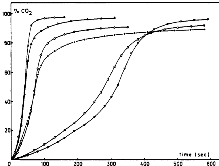
Fig. 1. \text{CO}_2 evolution curves; effect of dioxane used as cosolvent. No dioxane added to 100 parts MDI, 54 parts \text{H}_2\text{O} and 75 parts TCEP: (+) TMG (1.5 parts); ( \square ) 2MI (1.05 parts); ( \circ ) DMP (1.75 parts). 48 parts dioxane added to 100 parts MDI, 31 parts \text{H}_2\text{O} and 43 parts TCEP: ( \diamond ) TMG (1.5 parts); ( \nabla ) 2MI (1.05 parts); ( \Delta ) DMP (1.75 parts).
