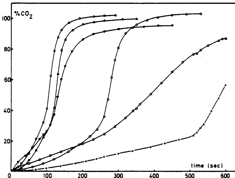
Fig. 2. \text{CO}_2 evolution curves; effect of dioxane used as cosolvent. No dioxane added to 100 parts MDI, 54 parts \text{H}_2\text{O} and 75 parts TCEP: (+) DABCO (1.5 parts); ( \square ) DMEA (2.1 parts); ( \circ ) DB (3.45 parts). 48 parts dioxane added to 100 parts MDI, 31 parts \text{H}_2\text{O} and 43 parts TCEP: ( \diamond ) DABCO (1.5 parts); ( \nabla ) DMEA (2.1 parts); ( \Delta ) DB (3.45 parts).
